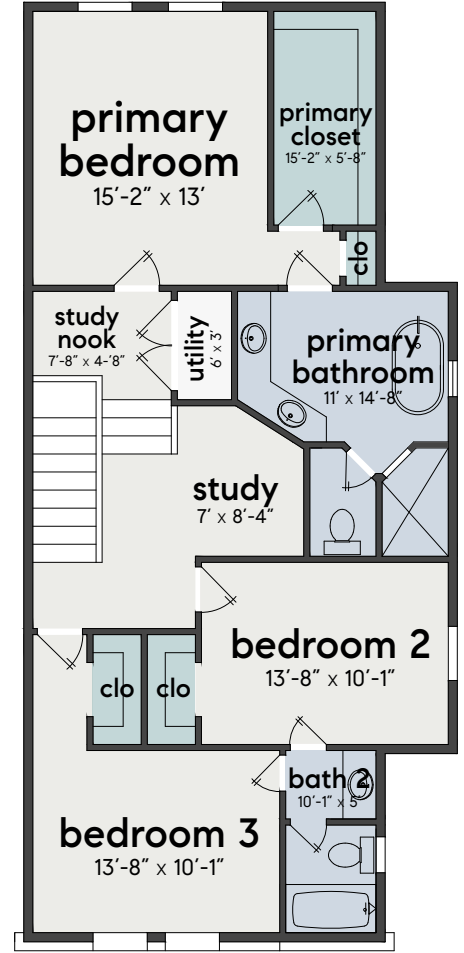
Second Floor Option 2
